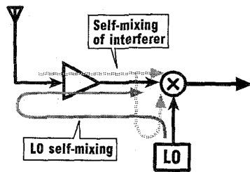
Fig. 9. Some sources of dynamic offset in a direct-conversion receiver. The LO may leak into the antenna, reflect off external objects, and downconvert to dc. A strong interferer may leak into the LO port and downconvert itself to dc. These dc offsets vary with physical location.
