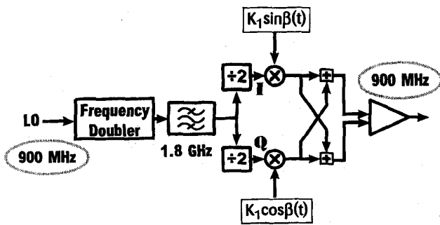
Fig. 14. A single-sideband upconversion circuit, where quadrature LO phases are derived by doubling LO frequency, and dividing down in \pm 2 flip-flops triggered on opposite edges. Quadrature baseband modulated signal is digitally synthesized. Sideband selection in final differential RF amplifier.
