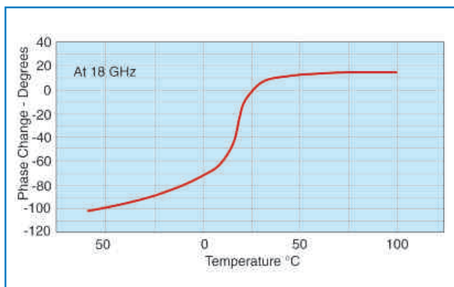
Fig. 10 Phase Stability
