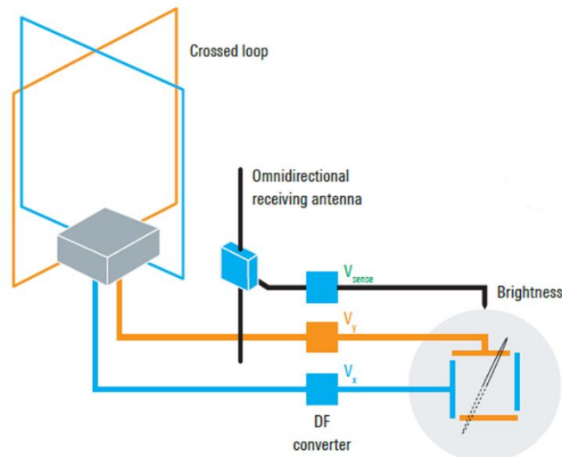
Figure 3 Working diagram of Watson-Watt Method
