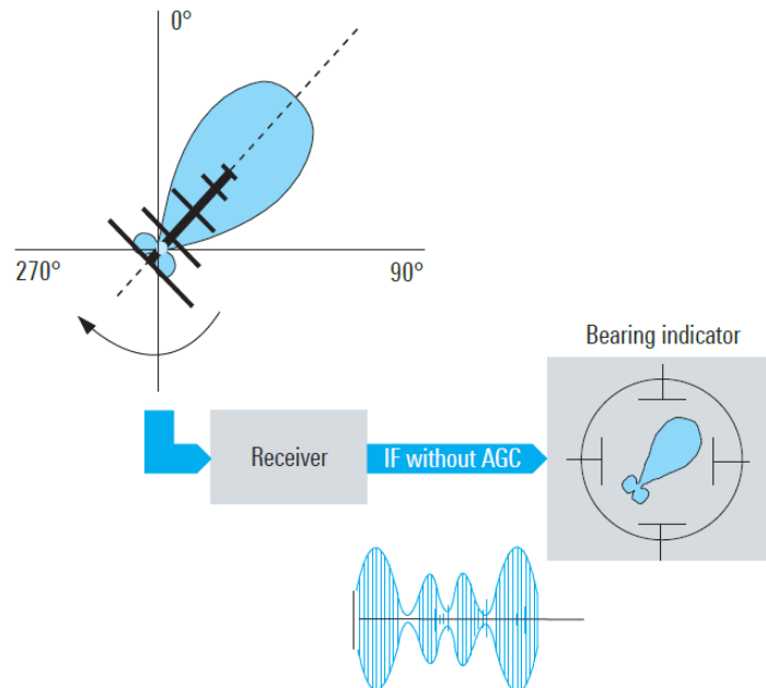
Figure 1 Direction finding using directional antenna.
