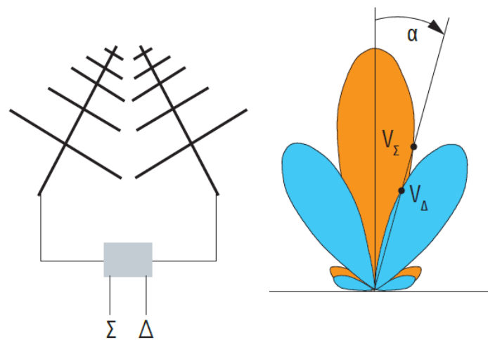
Figure 2 Direction finding using sum-difference method.
