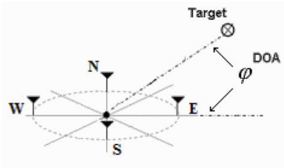
Figure 15 Adcock Antenna Array used for Watson-Watt Algorithm
