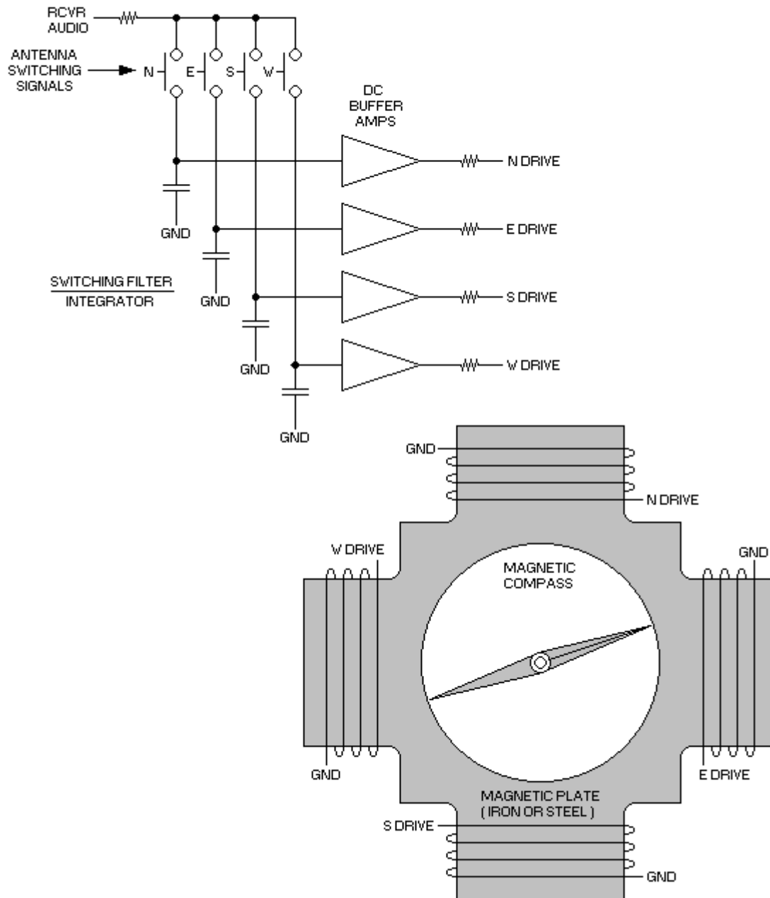
Figure 13 DF Resolver
