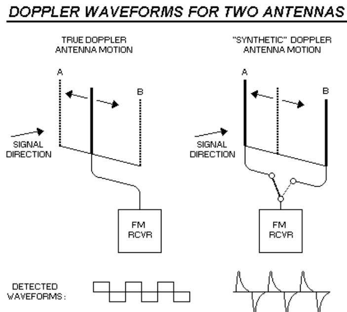
Figure 9 Doppler Waveform
