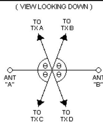
FIGURE 3 : BEARING AMBIGUITIES WITH A SINGLE ANTENNA PAIR
