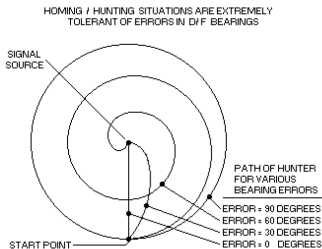
Figure 5 Bearing with 90, 60, 30 and 0 degree of errors.
