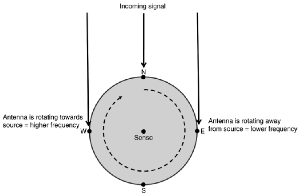
Figure 14 the figure shows a four-element pseudo-Doppler direction finding system. Each of the antenna will be turned on an off in N-E-S-W sequence.
