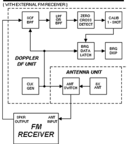
Figure 8 Doppler DF diagram
