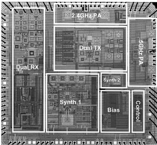
Fig. 17. Chip microphotograph.
