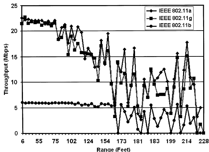
Fig. 25. Throughput/range of present design in IEEE 802.11a/b/g modes.
