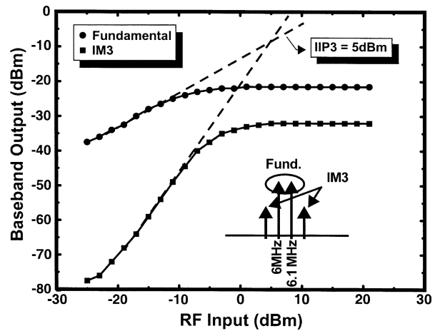
Fig. 19. Receiver intermodulation test.
