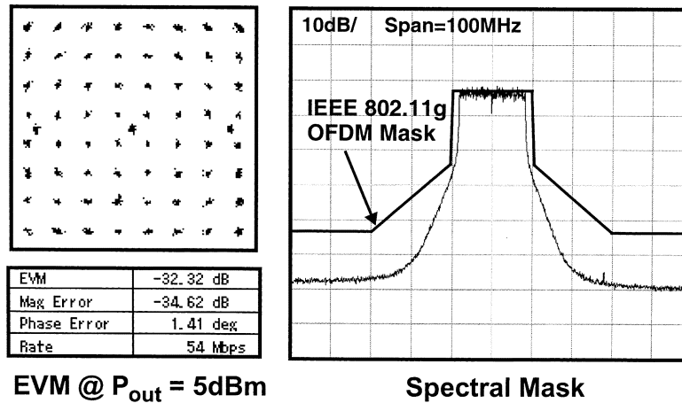
Fig. 20. Output spectrum and EVM of the 2.4-GHz transmitter.
