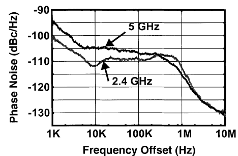
Fig. 23. Phase noise at the transmitter output.
