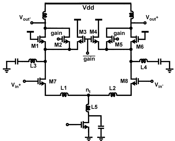
Fig. 4. Schematic of the 5-GHz LNA.
