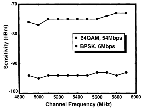
Fig. 18. Receiver sensitivity.
