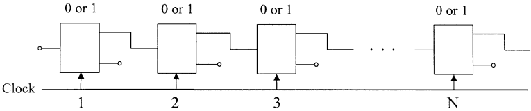
FIGURE 10.7 An m-sequence generator.
