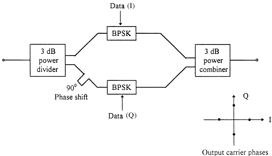
FIGURE 9.9 Quadriphase switch/modulator.
