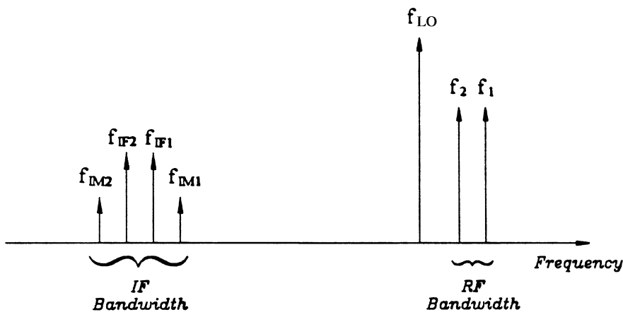
FIGURE 5.11 Intermodulation products.
