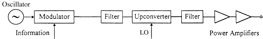
FIGURE 6.1 Transmitter system.
