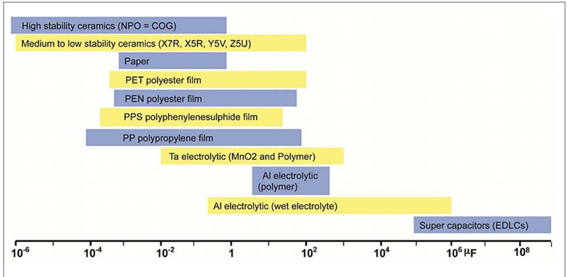
Figure 4: Values of capacitors by dielectric.
