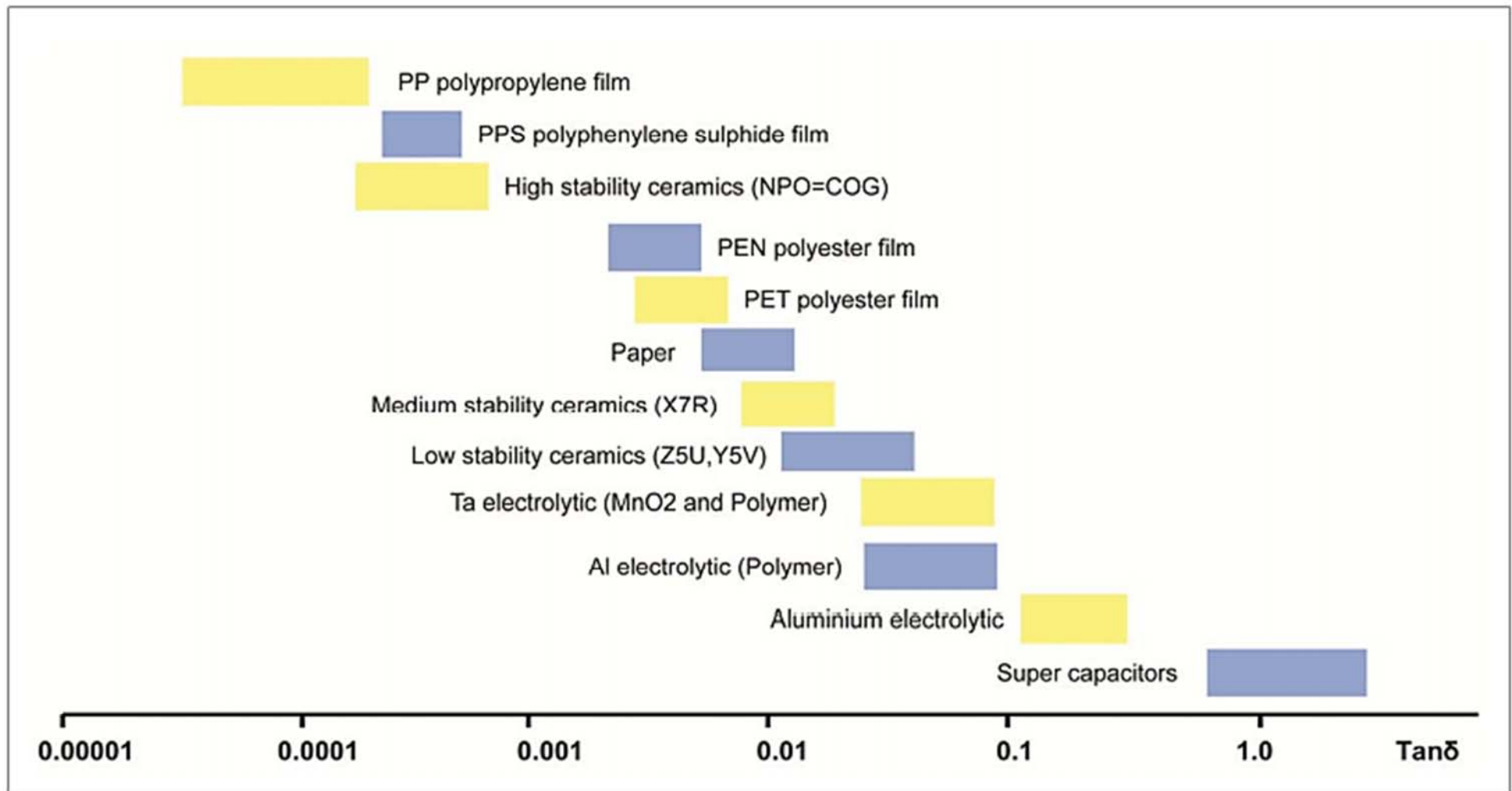
Figure 7: Dissipation factors ( \tan\delta ) of various dielectrics.
